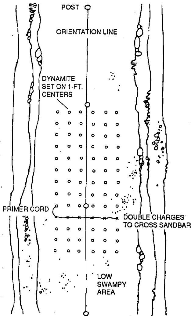
Top view of a ditching grid.
