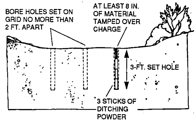
Side view of ditching set.
