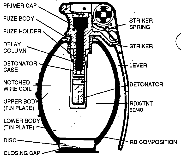
Current-issue British L2A2 antipersonnel hand grenade.
