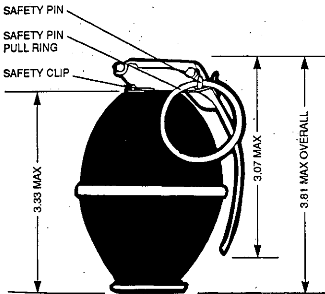
Standard-issue U.S. M61 delay-fragmentation hand grenade.
