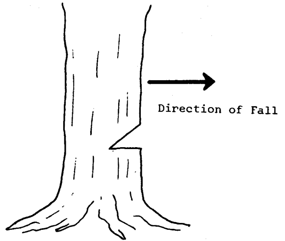
(b) Cut notch at approximately 45 degrees.
