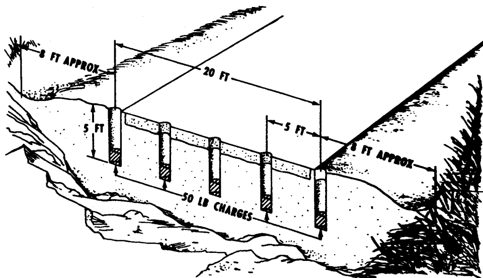
FIGURE 1 HASTY ROAD CRATER
