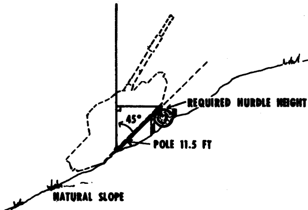
FIGURE 9 PROPER SITING OF A LOG HURDLE ON A SLOPE
