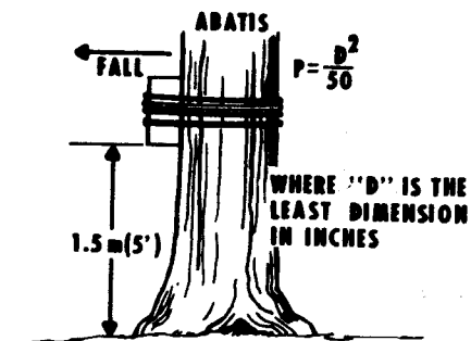
Figure 4 Charge Placement
