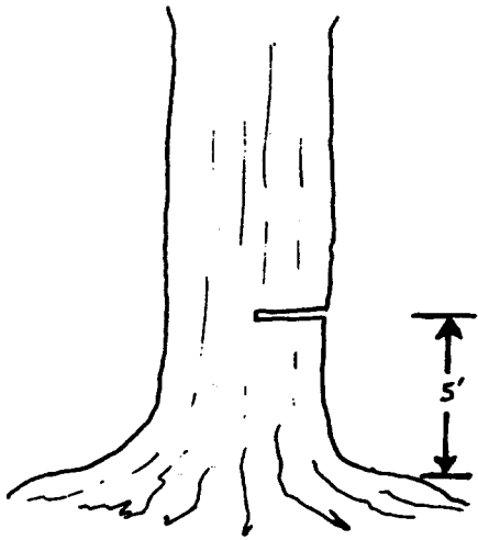
(a) Place undercut on the side of the tree in the direction of fall. (Less than half way through).
