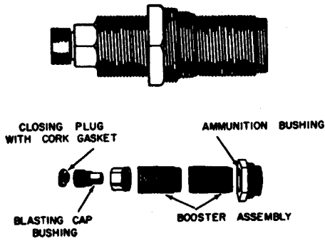
Figure 15 M10 Universal Explosive Destructor
