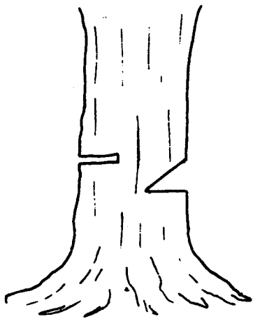
(c) Cut opposite side approximately 8" above undercut 1/3 way through.
