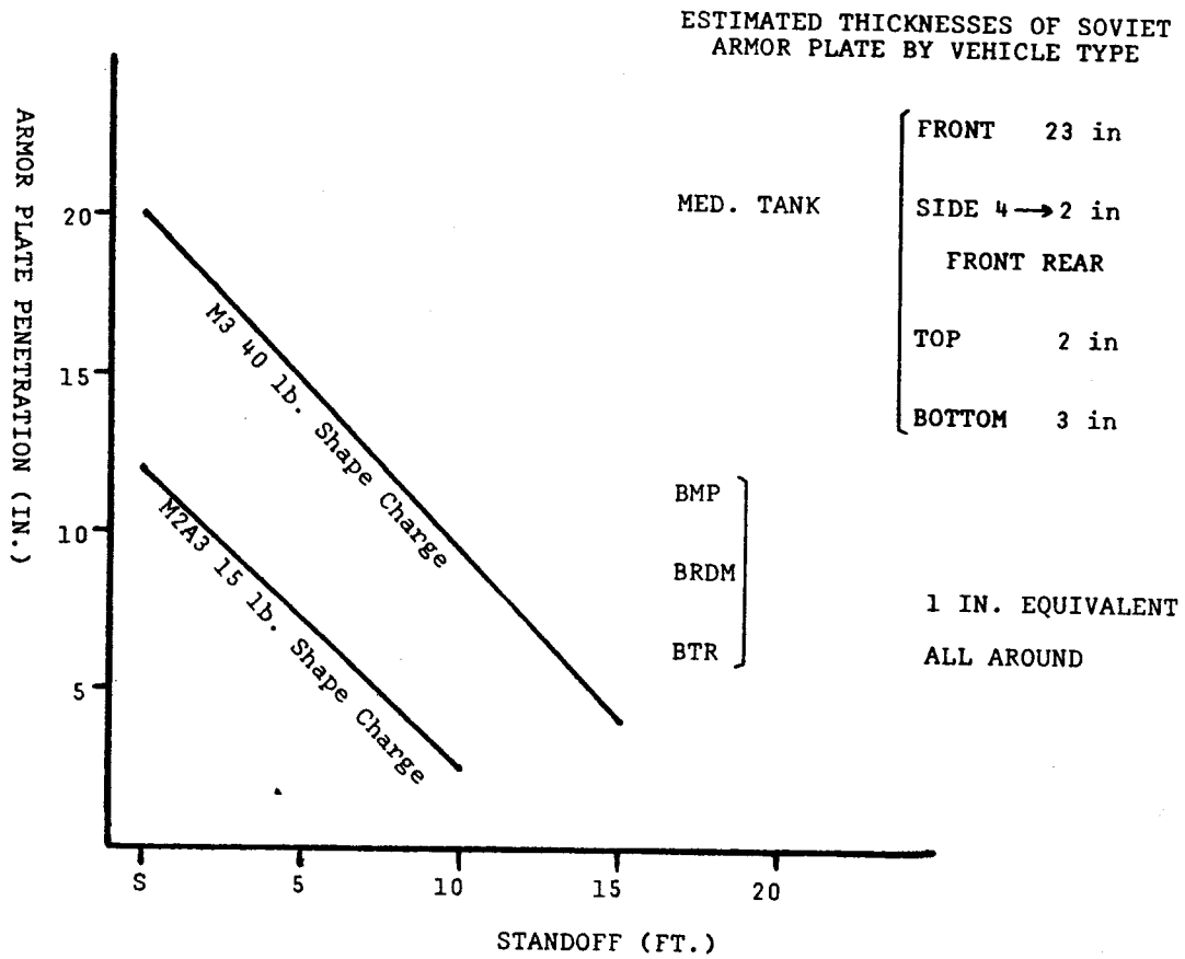
FIGURE 14 CONVENTIONAL SHAPE CHARGE EMPLOYMENT AGAINST ARMORED VEHICLES
