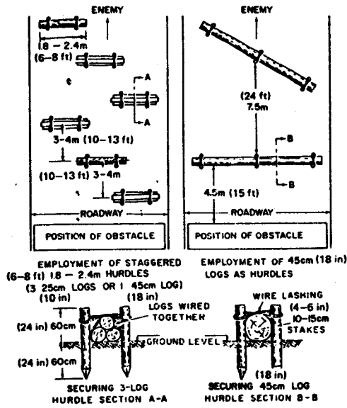
Figure 8 Type Log Hurdles
