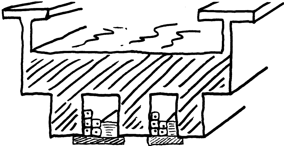
Figure 85. T-beam bridge.
