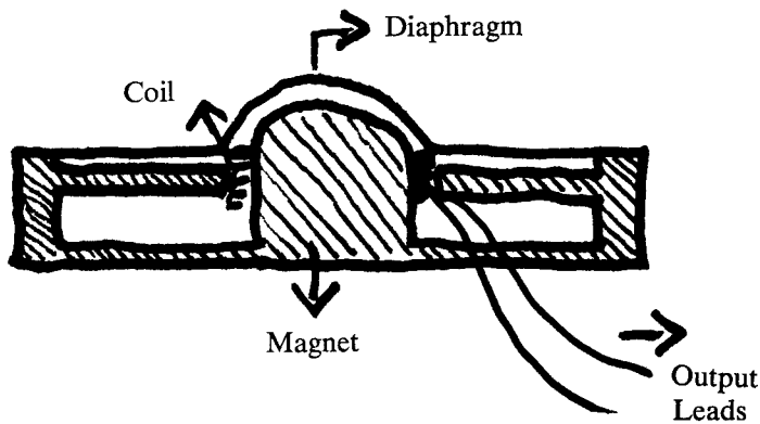
Figure 15. Dynamic Microphone.
