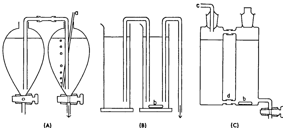
FIG. 10.3. (A, B, C) Devices for delivering mixed eluants in gradient elution.
