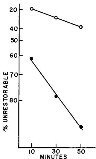
FIG. 3.11. "Aging" of plasma cholinesterase inhibited by DFP (○) or diisopropyl quinolinyl phosphate (●). Ordinate: % unresorable by 0.1M nicotindroxamic acid methiodide. Abscissa: time of contact of inhibitor and enzyme. From Hobbiger. 58
