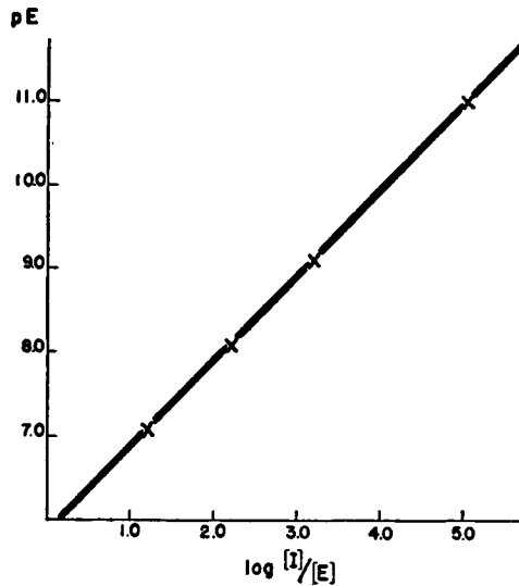
FIG. 3.3. Variation of [I]/[E] with pE , where [I] is DFP concentration for 50% inhibition of electric eel cholinesterase, [E] is enzyme concentration, pE is negative logarithm of enzyme concentration. From Nachmansohn et al. 76
