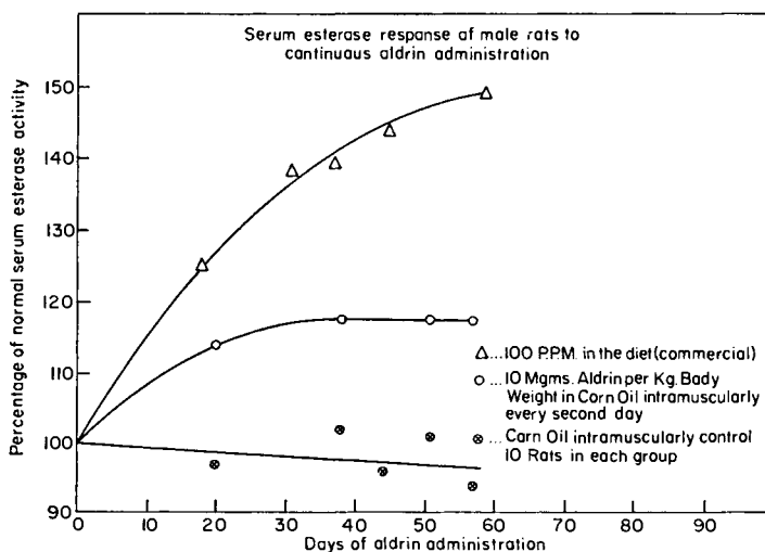
FIG. 6.9. Effect of aldrin feeding upon serum esterase levels in rats. From Crevier et al. 40
