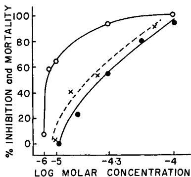
FIG. 7.1. Effects of DFP on the American cockroach. From Chadwick and Hill. 19
