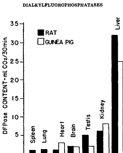
FIG. 4.1. "DFP-ase" content of homogenates of whole organs of the rat and guinea pig. From Mounter et al. 64
