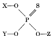
Phosphorothionate
