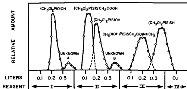
FIG. 10.2. Separation of the ionic metabolites of dimethoate on an ion-exchange column (Dowex 1). From Dauterman et al. 28
