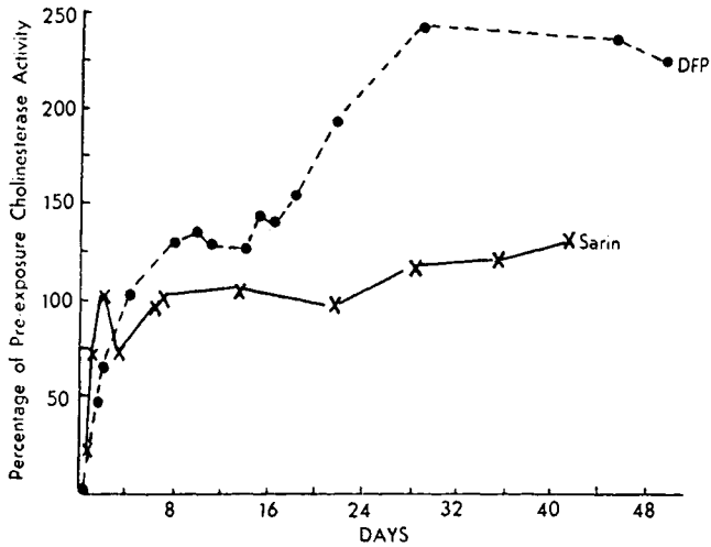
FIG. 6.2. Recovery of chicken plasma cholinesterase in vivo after treatment with DFP and sarin. From Austin and Davies. 14
