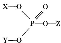
Phosphate
