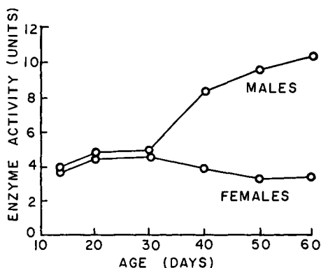
FIG. 4.5. Variation with age of Guthion-oxidizing activity in rat liver. From Murphy and DuBois. 69
