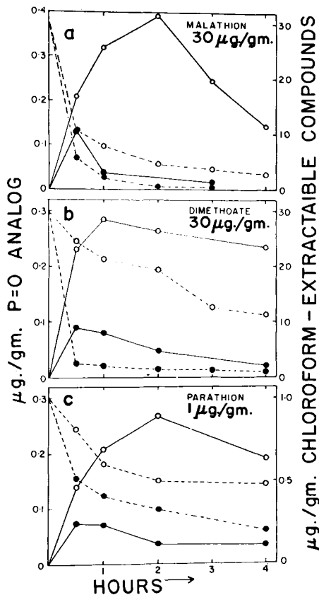
FIG. 9.1. (a, b, c). Levels of chloroform extractable compounds (---) and phosphate analog (—) in the American cockroach (○) and the mouse (●) after poisoning. The chloroform extractable compounds consist mainly of the parent compound, whose precise level may be obtained by subtracting the phosphate analog level from the chloroform-extractable level. From Krueger et al. 20, 21
