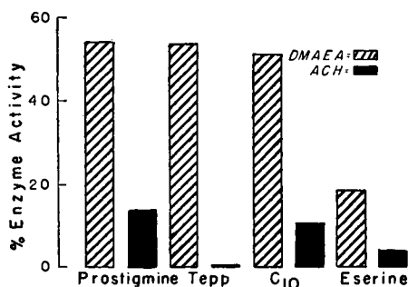
FIG. 6.6. Relative rates of hydrolysis by intact crab nerve of acetylcholine (ACH) and dimethylaminoethyl acetate (DMAEA), in the presence of various inhibitors. From Wilson and Cohen. 179
