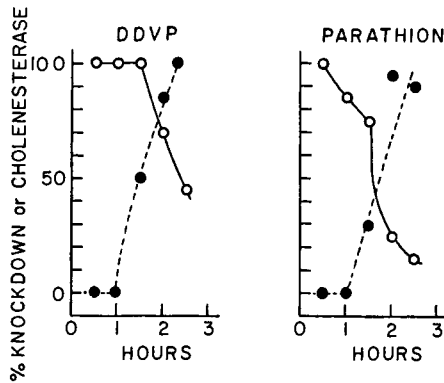
FIG. 7.3. Effect of DDVP and parathion upon knockdown and cholinesterase of whole houseflies. Flies were exposed to vapors of the insecticides. Plotted from data of van Asperen. 3
