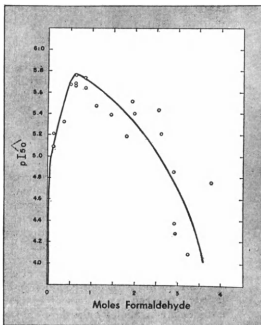
FIG. 3.8. Relationship between anticholinesterase activity and average degree of chlorination per mole of schradan, as measured by subsequent formaldehyde release. From Spencer and O'Brien. 89
