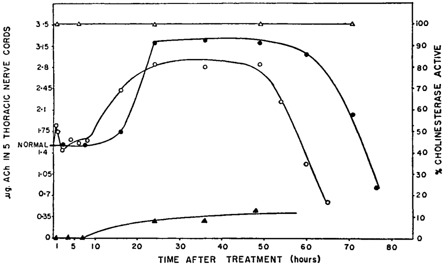
FIG. 7.5. Levels of cholinesterase and acetylcholine in the thoracic nerve cords of American cockroaches treated with TEPP (5 \mu\text{g.}/\text{gm.} ) or DDT (50 \mu\text{g.}/\text{gm.} ). From Colhoun. 28
