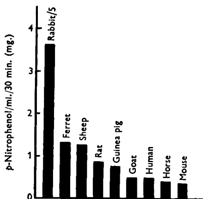
FIG. 4.3. Paraoxon-hydrolyzing activity of various sera. The value for rabbit has been reduced to one-fifth in the figure. From Aldridge. 5
