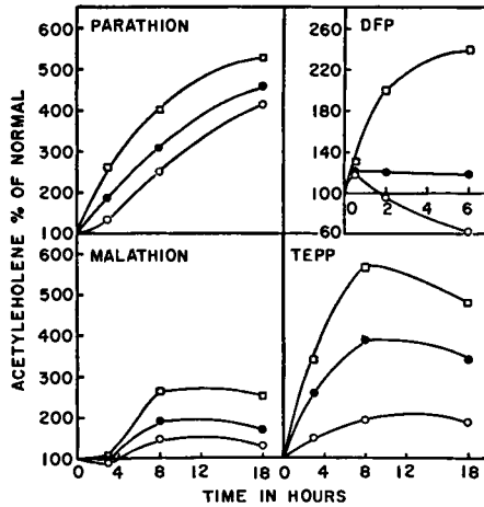
FIG. 7.4. Effects of organophosphates upon acetylcholine levels in houseflies. From Smallman and Fisher. 107 Dose about 50 \mu\text{g./gm} .
