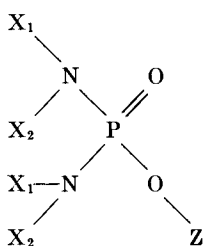
Phosphorodiamidate
