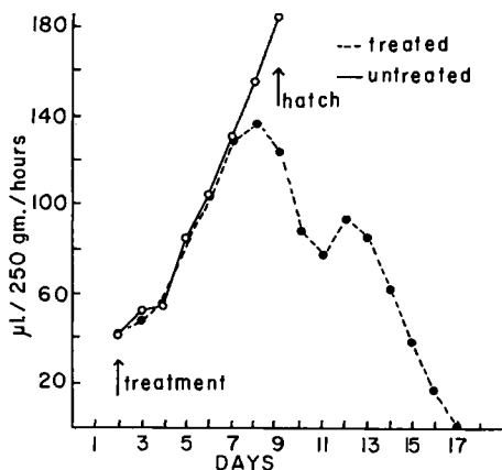
FIG. 7.6. Oxygen uptake by silkworm eggs and the effect of parathion treatment. From Staudenmayer. 114
