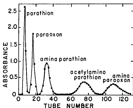
FIG. 10.1. Separation of parathion and some possible metabolites on a Celite column. From Ahmed et al. 1
