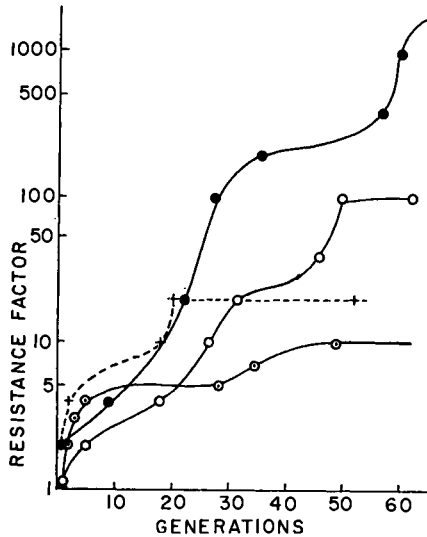
FIG. 7.9. Development of resistance to organophosphates by houseflies. The indicated insecticides were used to induce resistance and to test for it. Data plotted from March. 61
