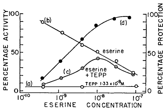
FIG. 3.9. Protection of erythrocyte cholinesterase by eserine against TEPP. (a) TEPP incubated for 20 minutes. (b) Eserine incubated for 20 minutes. (c) Eserine for 20 minutes followed by TEPP for 20 minutes. (d) % protection against TEPP by eserine. From Burgen. 23
