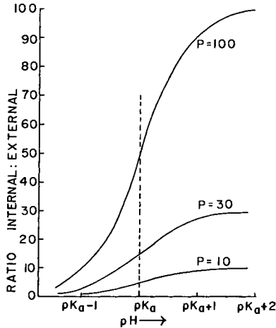
FIG. 5.3. Penetration of bases into a lipid from an aqueous phase. P = partition coefficient, internal (lipid) phase: external (aqueous) phase. Ratio on ordinate is that of molar concentrations.
