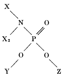
Phosphoramidate
