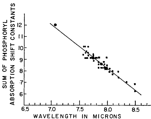
FIG. 10.4. Relationship between the wavelength of infrared absorption for P=O and the electronegativity of substituents, in pentavalent organophosphates. From Bell et al. ? ●: Values for F_3P(O) , Cl_3P(O) , and Br_3P(O) on which the values for the shift constants were based.
