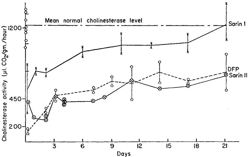
FIG. 6.3. Recovery of chicken spinal cord pseudocholinesterase in vivo after treatment with DFP and sarin. From Austin and Davies. 14
