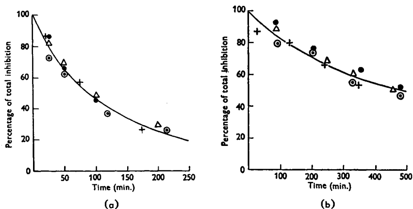
FIG. 3.1. Rate of reactivation of phosphorylated cholinesterase. (a) Erythrocyte cholinesterase with dimethyl phosphates: +, dimethyl p -nitrophenyl phosphate; ●, dimethyl phosphoric anhydride; ⊙, dimethyl phosphorofluoridate; Δ, O,O -dimethyl S-p -nitrophenyl phosphorothiolate. (b) Serum cholinesterase with diethyl phosphates: +, paraoxon; ●, TEPP; Δ, diethyl phosphorofluoridate; ⊙, parathion, S -phenyl isomer. From Aldridge and Davison. 9
