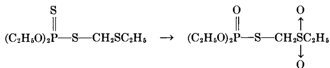
Thimet
