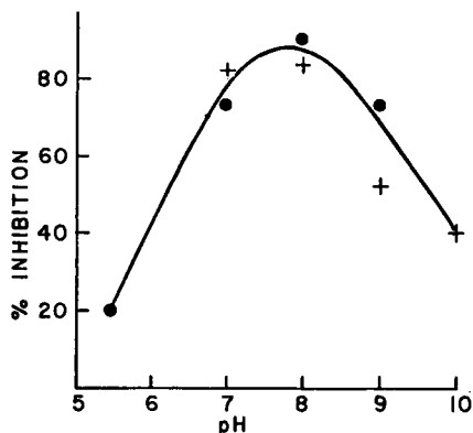
FIG. 3.4. Relationship between pH and inhibition of acetylcholinesterase by TEPP. From Wilson and Bergmann. 100
