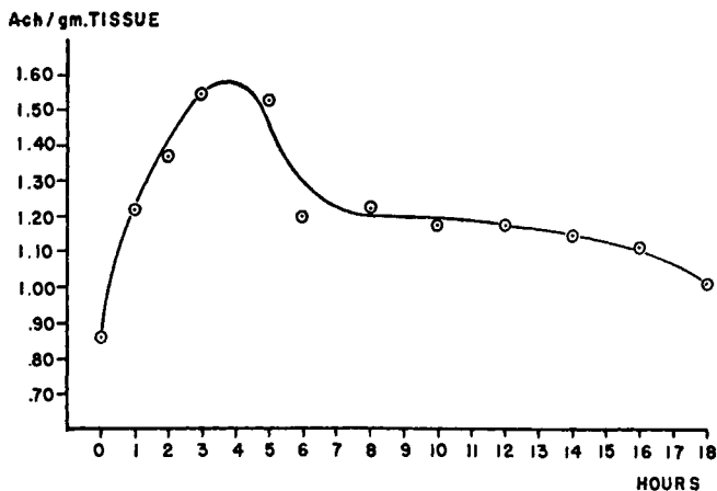
FIG. 6.8. Acetylcholine in rabbit brain cortex after DFP, 0.4 mg./kg. intravenously. From Michaelis et al. 127
