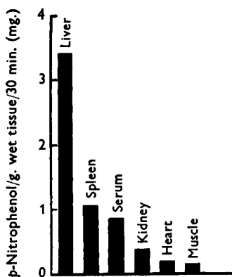
FIG. 4.4. Paraoxon-hydrolyzing activity of rat tissue homogenates. Activities of pancreas, brain, and submaxillary gland were undetectable. From Aldridge. 5
