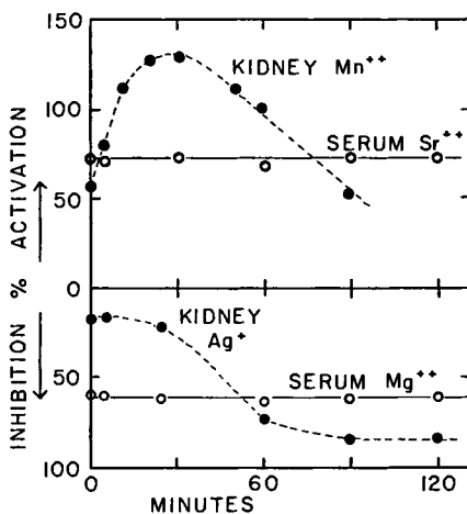
FIG. 4.2. Variation with time of the effects of salts upon "tabunase" from human serum or pig kidney. From Augustinsson and Heimburger. 16
