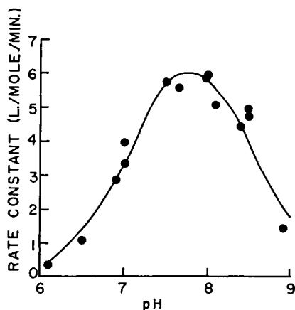
Fig. 3.10. Reactivation of diethyl-phosphorylated cholinesterase by MINA at different pH values. From Davies and Green. 32
