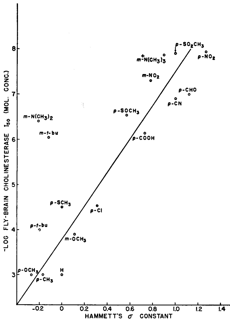
FIG. 3.6. Relationship between anticholinesterase activity and Hammett's \sigma constants for substituted diethyl phenyl phosphates. From Fukuto and Metcalf. 40
