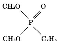
Dimethyl ethylphosphonate
