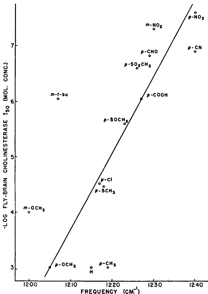
FIG. 3.7. Relationship between anticholinesterase activity and infrared P-O-aromatic stretching frequency for substituted diethyl phenyl phosphates. From Fukuto and Metcalf. 40
