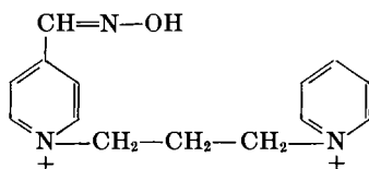
1-(4-Hydroxyiminomethylpyridinium)-3-pyridinium propane
