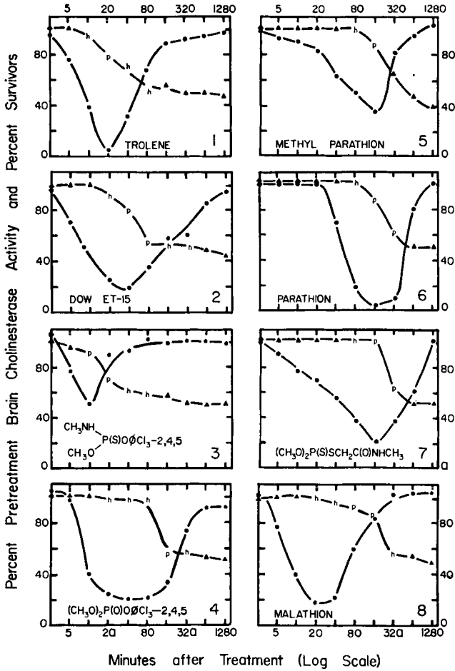
FIG. 7.2. Effects at varying times of organophosphates upon surviving houseflies. From Mengle and Casida. 67 Dose: 24 hours LD 50
