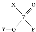
Phosphonofluoridate
