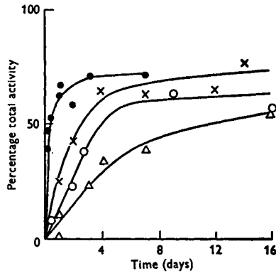
FIG. 6.1. The recovery of inhibited rat brain cholinesterase in vivo . Each point represents the mean brain time cholinesterase activity of two rats. Dimethyl (●), diethyl (X), di- n -propyl (O), diisopropyl and diisopropylamino (Δ) substituted phosphates were used in these experiments. From Davison. 50
