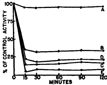
FIG. 6.4. Effect of symmetrical diethyl bis(dimethylamido) pyrophosphate upon rat cholinesterases in vivo . Curve A, brain; Curve B, skeletal muscle; Curve C, ileum; Curve D, submaxillary gland; and Curve E, serum. From DuBois et al. 67
