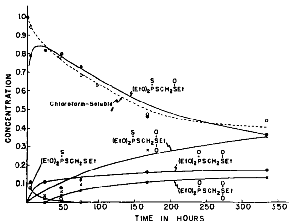
FIG. 8.3. Thimet metabolism in isolated cotton leaves. Labeling as in Fig. 8.1. From Metcalf et al. 73
