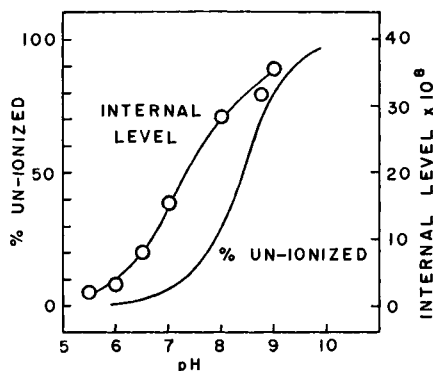
FIG. 5.1. Penetration of Tetram into the intact American cockroach nerve cord. The curve on the left indicates the molar concentration of Tetram inside the cord (scale on right of figure). The other curve is a dissociation curve plotted for a pK_a of 8.4 (scale on left of figure). The ordinates are on scales arbitrarily selected to make the curves the same height.
