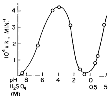
FIG. 2.2. Relationship between pH and hydrolysis constant for 1-methoxypropyl-2-phosphate
