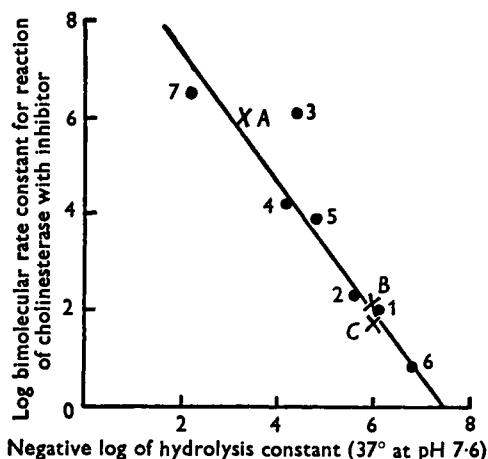
FIG. 3.5. Relationship between hydrolyzability and anticholinesterase activity for ten substituted diethyl phenyl phosphates. From Aldridge and Davison. 8
