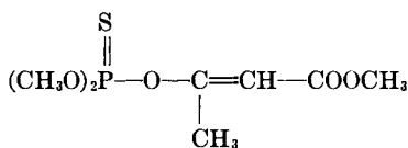
Thiono-Phosdrin
