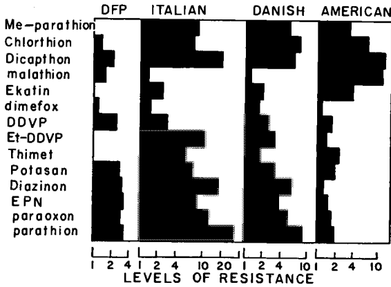
FIG. 7.10. "Resistance spectra" of four housefly strains. Level of resistance = (LD_{50} \text{ resistant}) / (LD_{50} \text{ susceptible}) . From Busvine. 16
