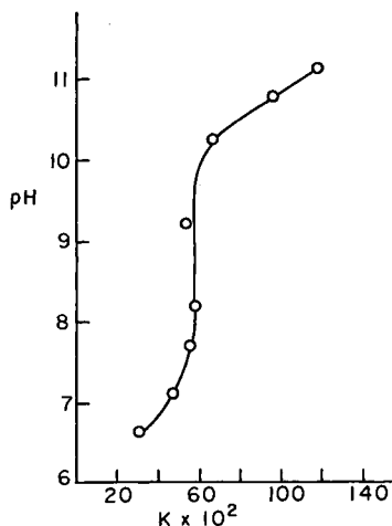
FIG. 2.3. Relationship between pH and hydrolysis constant for DFP in the presence of \text{CuSO}_4 and dipyrldyl (1:1) at 30^\circ\text{C} . From Wagner-Jauregg et al. 88
