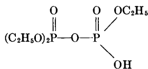
Triethyl pyrophosphate
