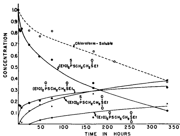
Fig. 8.1. Disyston metabolism in isolated cotton leaves. Chloroform-soluble: fraction of total radioactivity extractable into chloroform. Others: fraction of chloroform-soluble material as indicated metabolite. From Metcalf et al. 73
