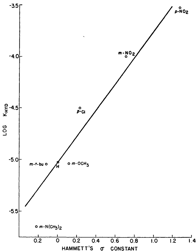
FIG. 2.1. Relationship between hydrolyzability (as log of hydrolysis constant, k ) and Hammett \sigma constant, in substituted diethyl phenyl phosphates. From Fukuto and Metcalf. 30
