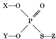
Phosphorothiolate
