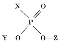
Phosphonate
