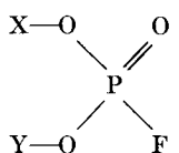
Phosphorofluoridate
