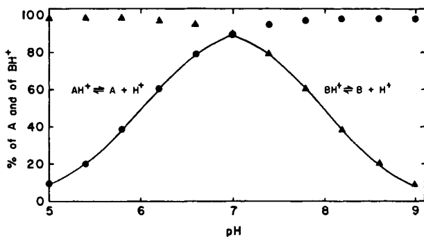
FIG. 1.1. Variation with pH of production of A from AH^+ (circles) and of BH^+ from B (triangles), when the acid AH^+ has a pK_a of 6.0, the base B a pK_a of 8.0. The line gives the amount of (A + BH^+) as a function of pH; the amount is maximal at the mean pK_a .
