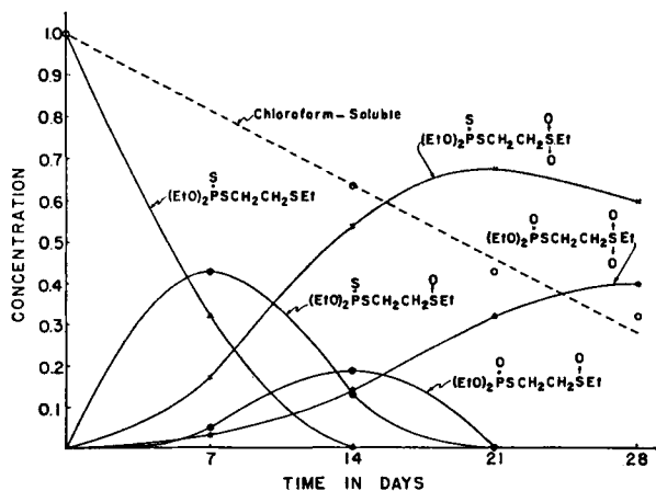
Fig. 8.2. Disyston metabolism in alfalfa plants after seed treatment. Labeling as in Fig. 8.1. From Metcalf et al. 73
