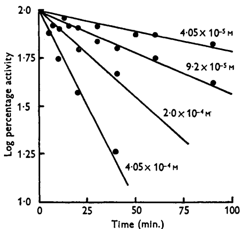
FIG. 3.2. Rate of inhibition of erythrocyte cholinesterase by purified diethyl p -chlorophenyl phosphate. From Aldridge and Davison. 7
