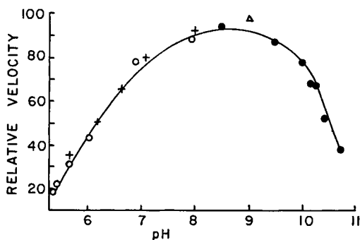
FIG. 1.2. Acetylcholine hydrolysis by purified electric eel acetylcholinesterase as a function of pH. From Wilson and Bergmann [ J. Biol. Chem. 186 , 683 (1950)].
