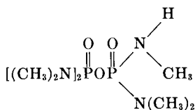
Heptamethylpyrophosphoramidate (HMPA)
