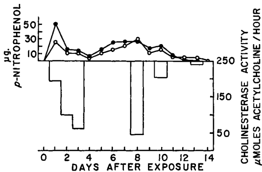
FIG. 6.5. Serum cholinesterase and urinary p -nitrophenol in a monkey poisoned dermally with parathion. From Waldman et al. 173
