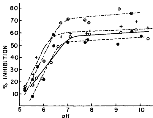
FIG. 1.3. Inhibition of purified electric eel acetylcholinesterase by quaternary ammonium salts as a function of pH. From Bergmann and Shimoni. 14
