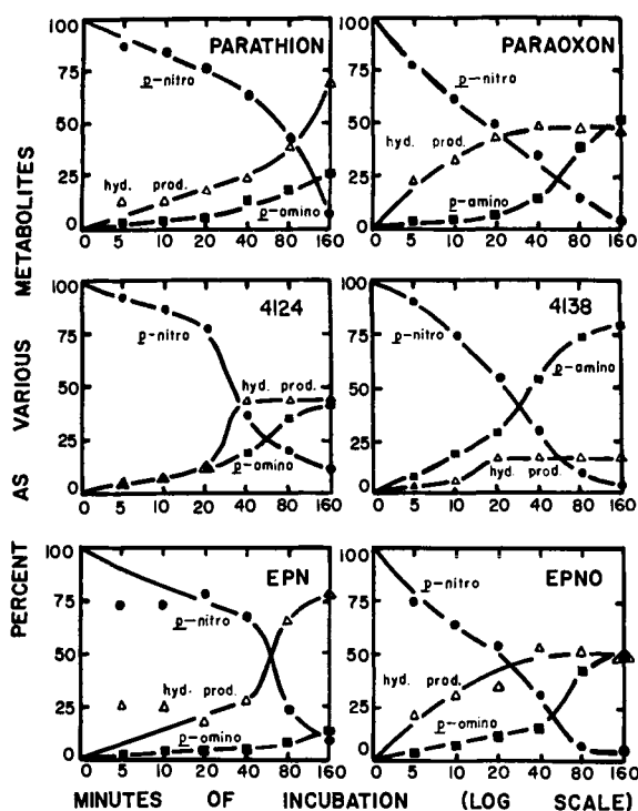
FIG. 6.10. Hydrolysis and reduction of organophosphates by stagnating bovine rumen juice. All compounds at 300 p.p.m. From Ahmed et al. 2
