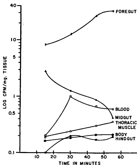
FIG. 7.8. Concentration of radioactivity in American cockroach tissues after applying labeled TEPP topically. Dose probably about 15 \mu\text{g./gm.} From Roan et al. 99
