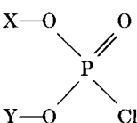
Phosphorochloridate
