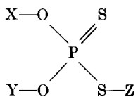
Phosphorodithioate
