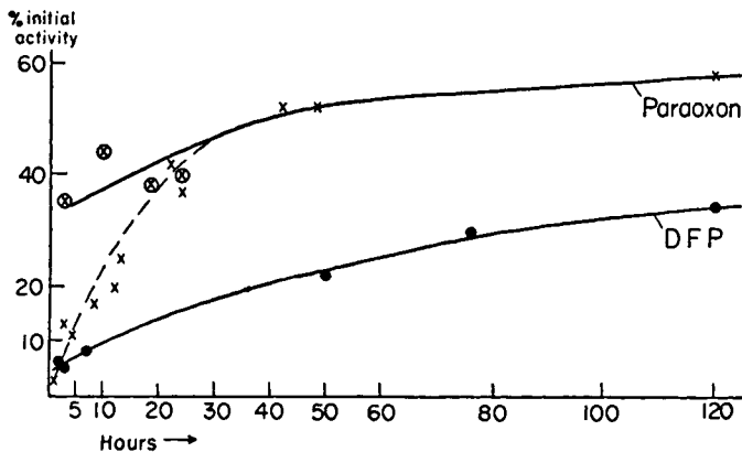
FIG. 6.7. Spontaneous recovery of acetylcholinesterase activity in the brain of mice after subcutaneous injection of paraoxon or DFP ( LD_{50} dose). Chloroform extraction used (see text) for all except the paraoxon \times — \times data. From Kewitz and Nachmansohn. 100
