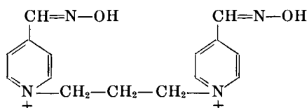
1,3-Di(4-hydroxyiminomethylpyridinium)propane
