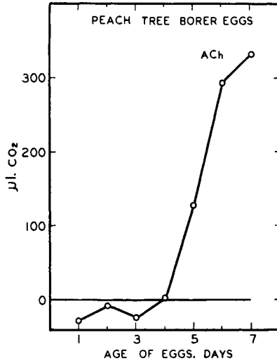
FIG. 7.7 Occurrence of cholinesterase in peachtree borer eggs of various ages. Ordinate shows \mu\text{l. CO}_2 released in 180 minutes by a homogenate of 2000 eggs, using manometric assay. From Smith. 110
