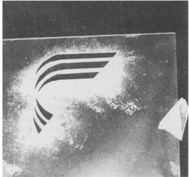
Made a stencil of the New Jersey logo out of Dura-Lar film.
