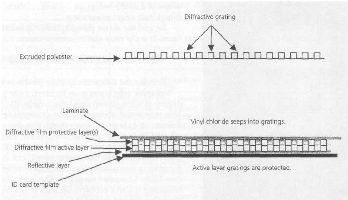
Illustration 1 shows the various layers of a diffractive film hologram ID. It shows a second layer of film to protect the first and a reflective layer beneath the first layer of film. It is possible to have only one layer of film, an "active" layer, upside down and cold-laminated (or very carefully heat-laminated). Also, the reflective layer need not be a separate metallized layer. A glossy template may have sufficient reflectivity without metallization.
