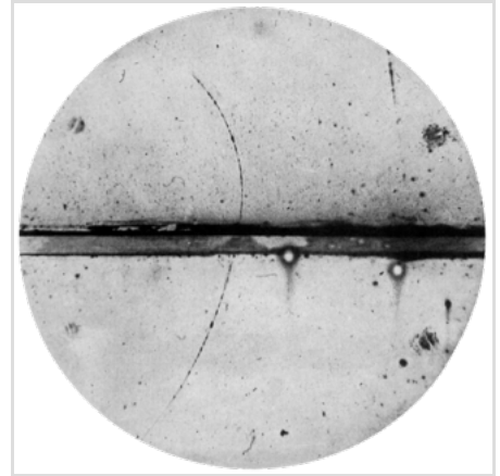
A cloud chamber photograph of the first observed positron , 2 August 1932.
